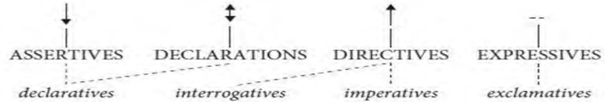
Figure 1. Searle's classification of illocution types
