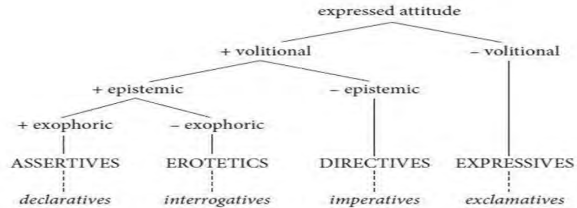
Figure 2. Zaefferer's classification of illocution types
